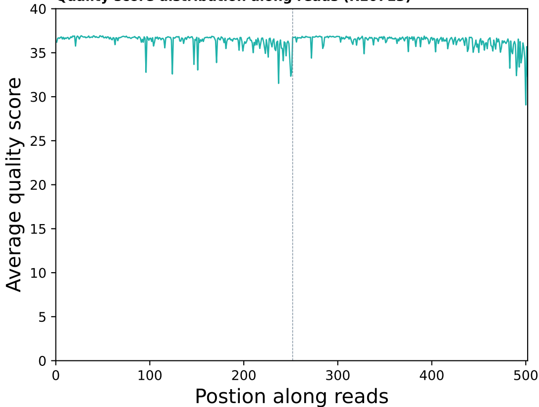
Quality score distribution along reads (R10713)
